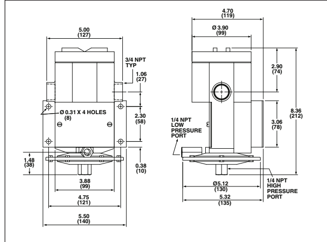
P-Series Dimension Drawing – 70A1884
