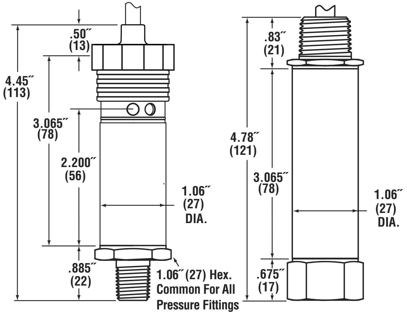
A2 Dimension Drawing
