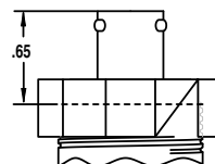
(4) PIN BEND STYLE ELECTRICAL TERMINATION SHELL SIZE 8
