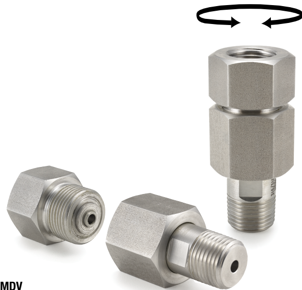
MDV Swivel Adapter
