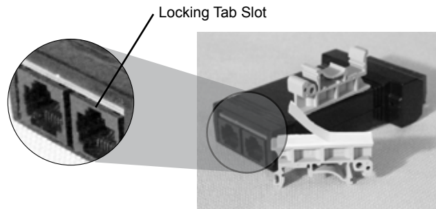
Figure 2. DIN Rail Clips Mounted to Expansion Module
