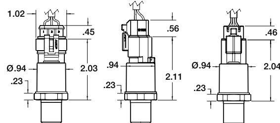
3-PIN METRI-PACK®*
